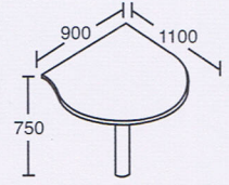
RE-CT1100 Connection Top with Metal Leg (Left & Right) L1100 x W900 x H750
