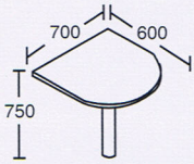
RE-HRCT70 Half Round Connection Top with Metal Leg L600 x W700 x H750
