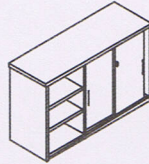
WN-SBC1200 Side Board Cabinet L1200 x W400 x H750
