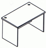
IR-1200 Writing Table L1200 x W700 x H750
