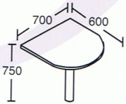
IR-HRCT70 Half Round Connection Top with Metal Leg L600 x W700 x H750
